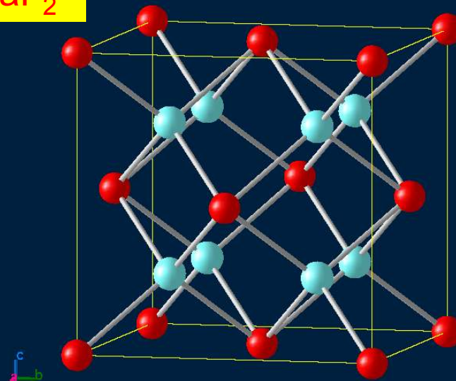
CaF 2
