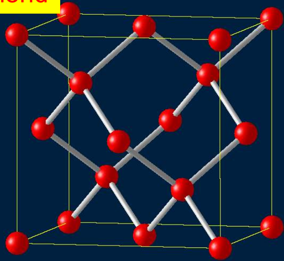
Diamond
