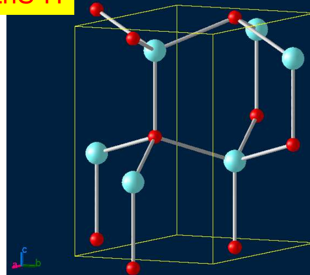
ZnS-H
